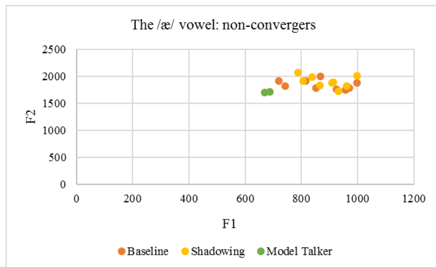
Graph 2. Formant Values for the /æ/ for Non-Convergers
